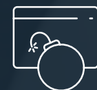
DDoS attacks
